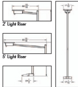
Surface Mount Base
